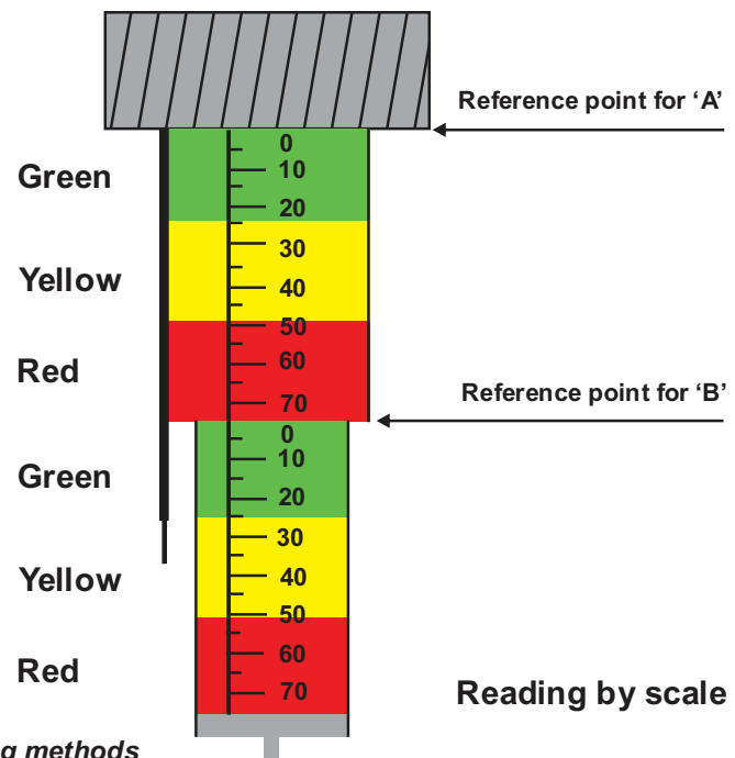
Dual height tell-tale general assembly
